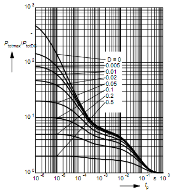
Permissible Pulse Load P_{totmax} / P_{totDC} = f(t_p)
