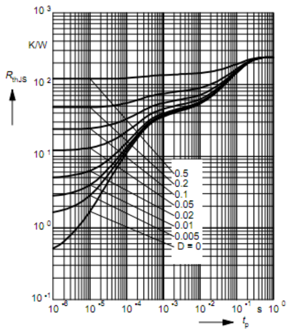
Permissible Pulse Load R_{thJS} = f(t_p)
